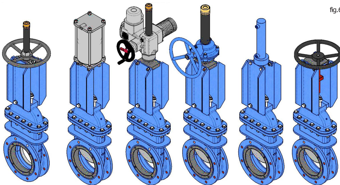
Handwheel with rising stem
